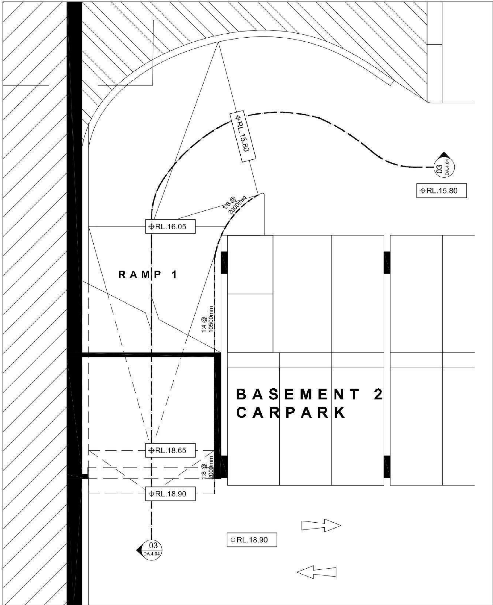
02 RAMP 1 PLAN BASEMENT 2 DETAIL
