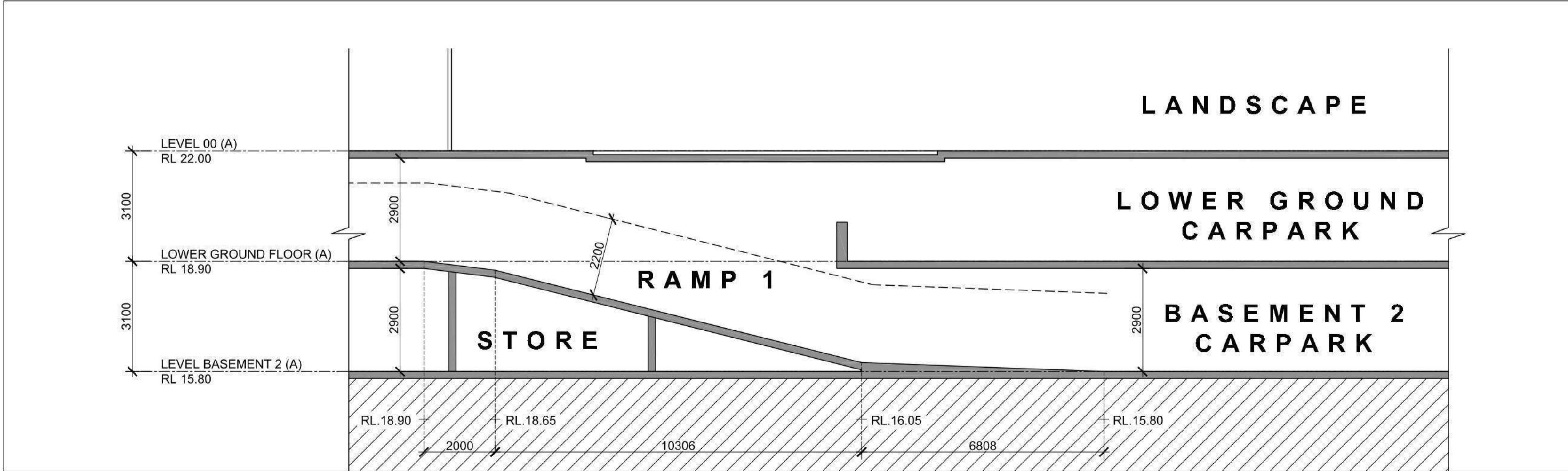
03 RAMP 1 SECTION
