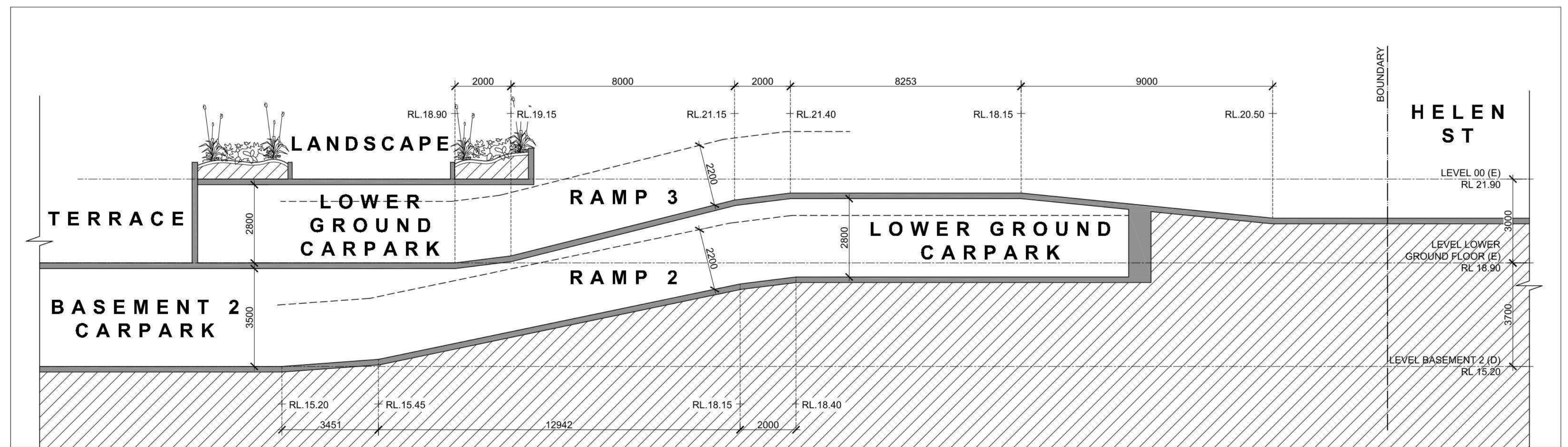
04 RAMP 2+3 SECTION
