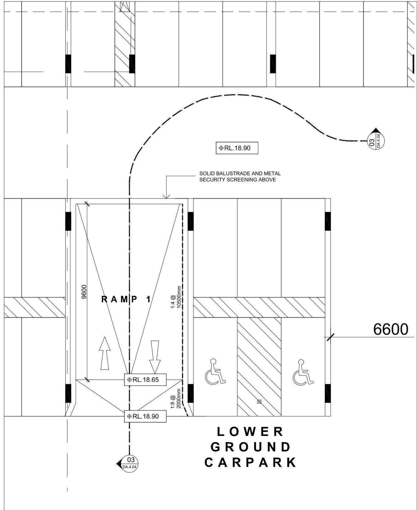
01 RAMP 1 PLAN LOWER GROUND FLOOR DETAIL
